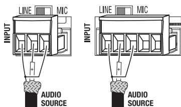
Figure 2.4.1 Input Wiring
