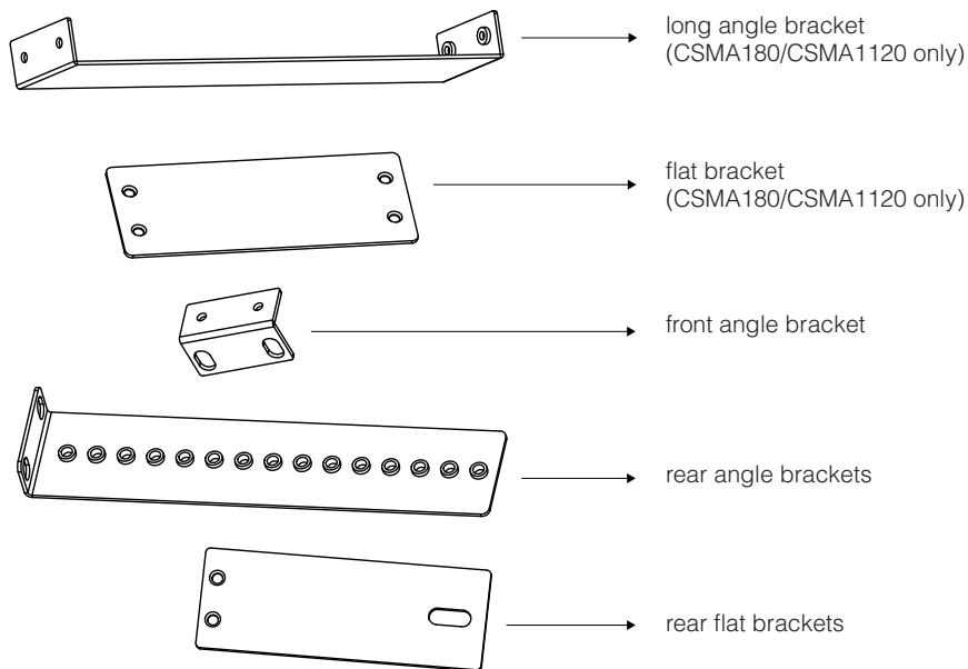
Figure 2.2.2 Mounting Kit
